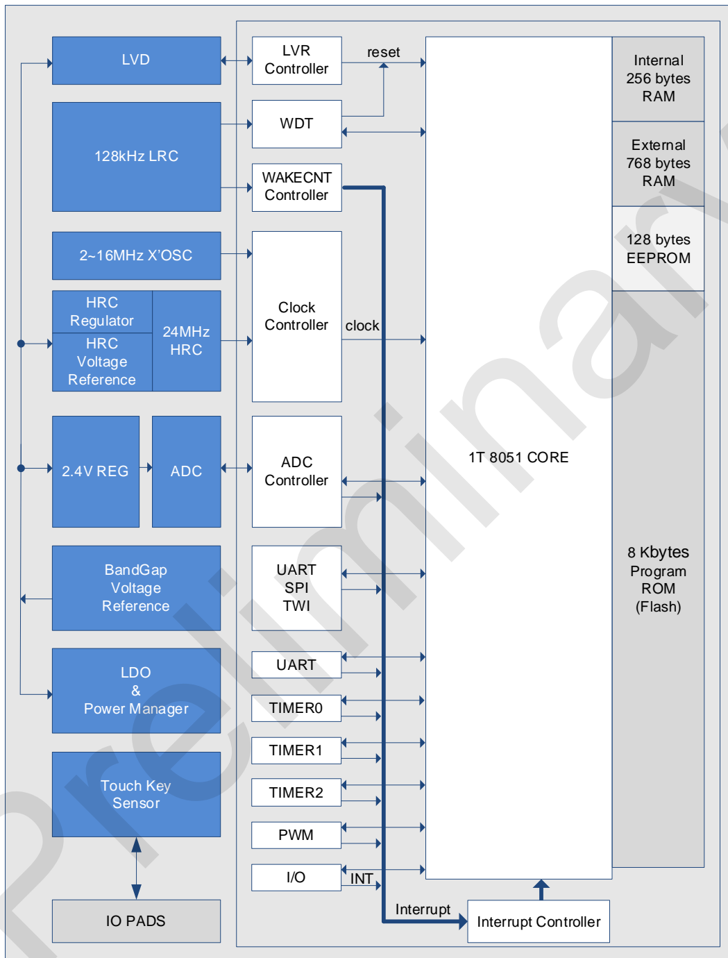
The SC92F83AX BLOCK DIAGRAM
