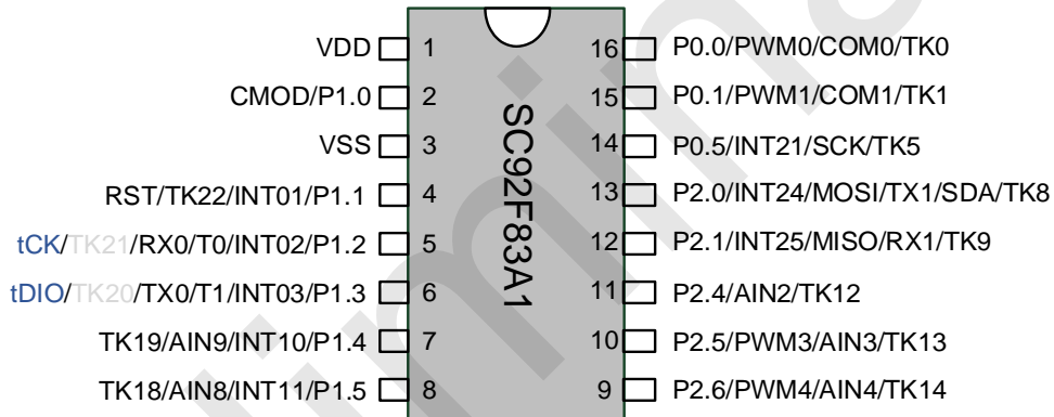
The SC92F83A1 Pin Diagram
