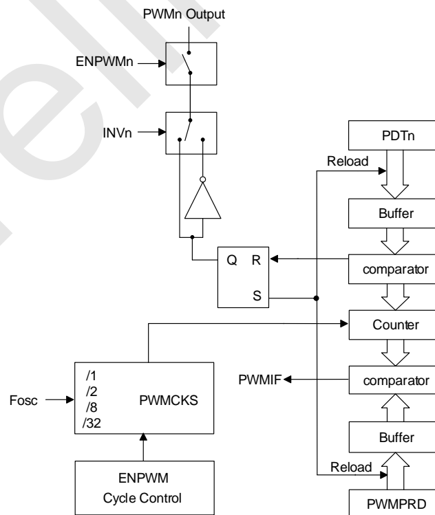
The SC92F83AX PWM Independent Mode Block Diagram
