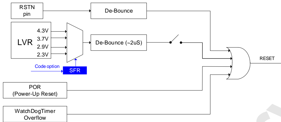
The SC92F83AX Reset Diagram
