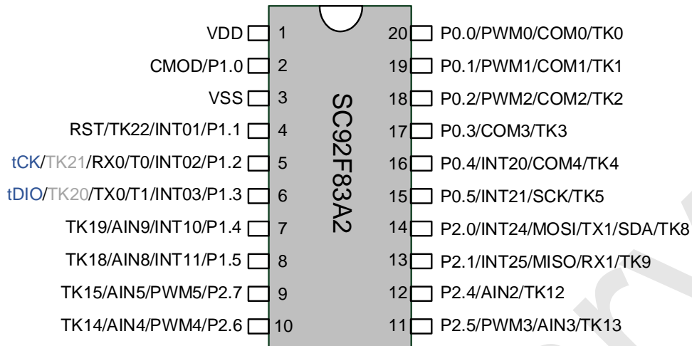
The SC92F83A2 Pin Diagram
