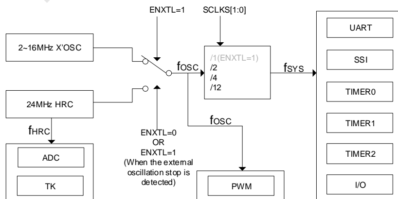
The SC92F83AX Internal Clock Relationship
