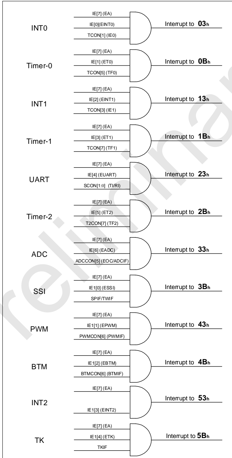
The SC92F83AX Interrupt Structure and Vector
