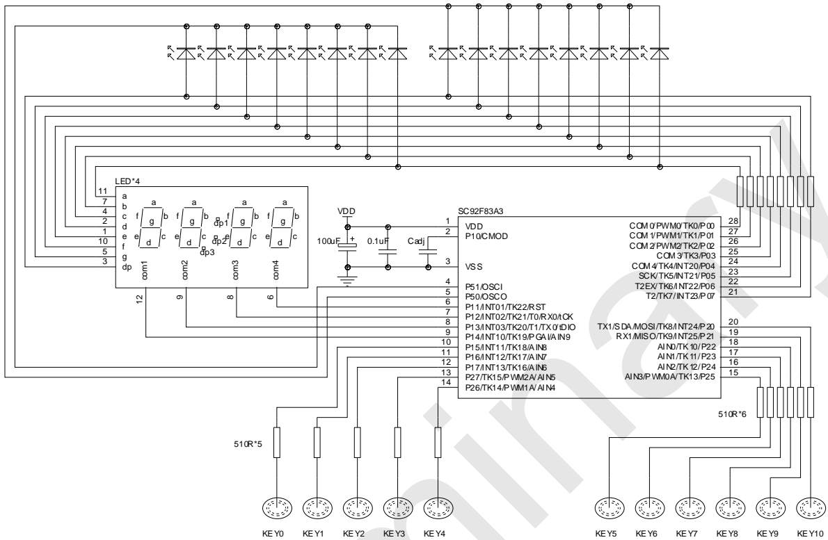
The SC92F83A3 TouchKey Application Circuit Diagram
