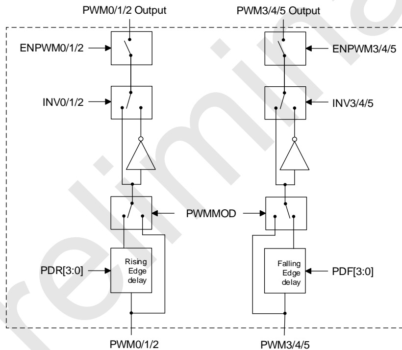
The SC92F83AX PWM Complementary Mode Block Diagram
