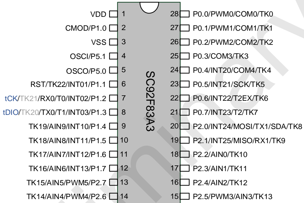
The SC92F83A3 Pin Diagram
